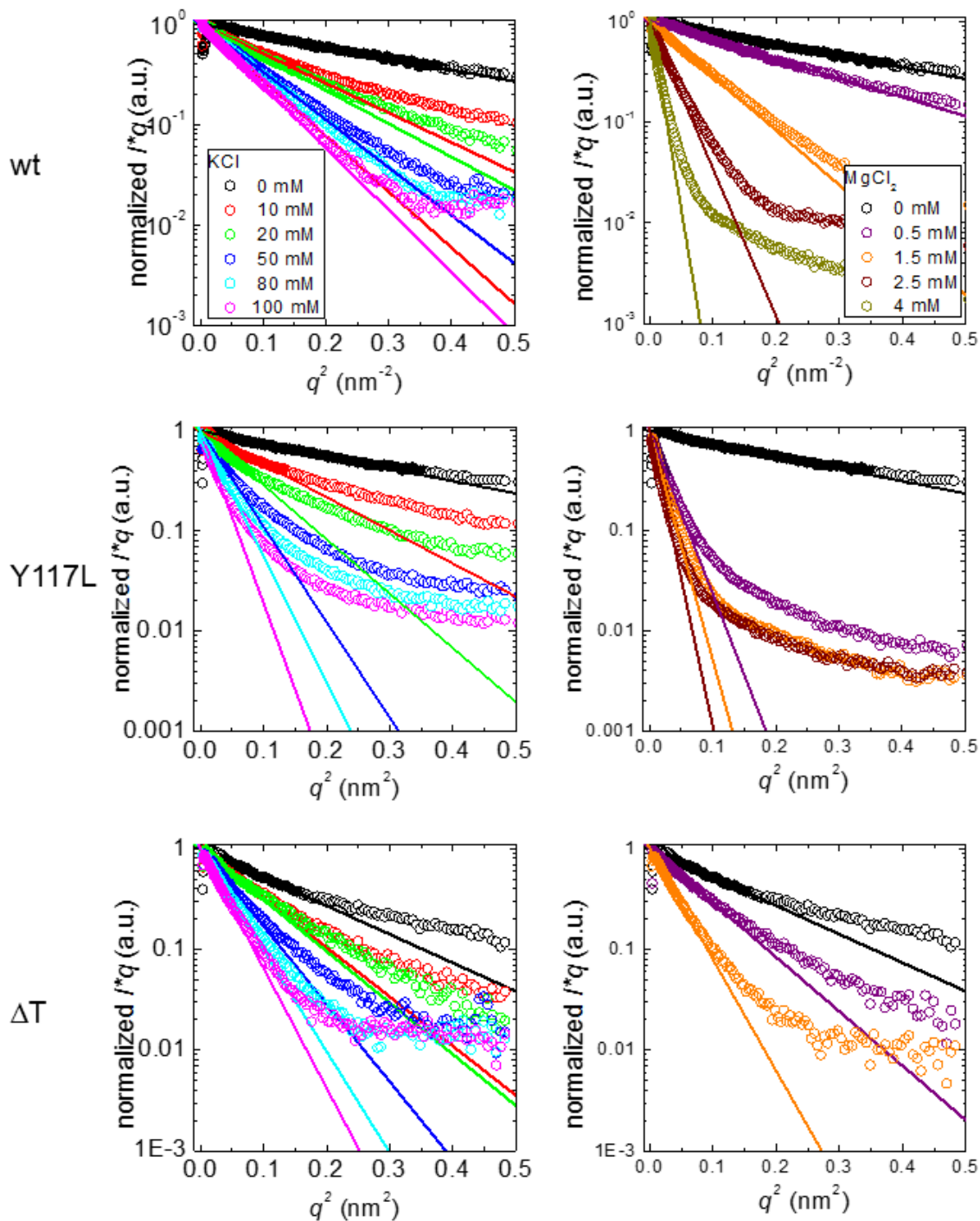
Figure S1. Guinier fits for all ionic conditions presented in the main text in Figure 3, also including the wt data.
